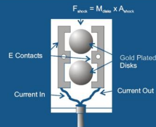
SP3237 Shock Sensor
